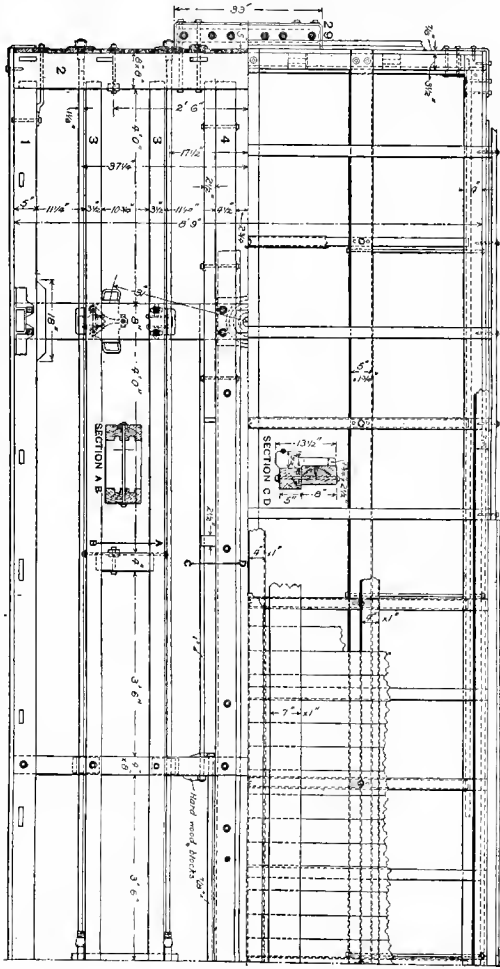
Fig. 245. Half Plan showing Roof and Underframing.
